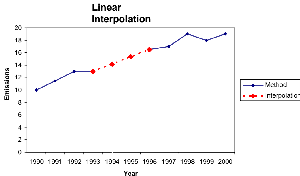
Figure 2-3 Linear interpolation
